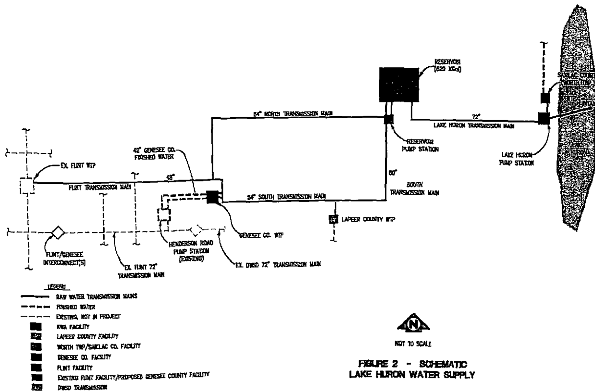
Figure 2: Schematic Lake Huron Water Supply
