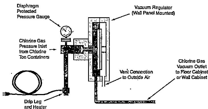
Figure 4: Vacuum Regulator
