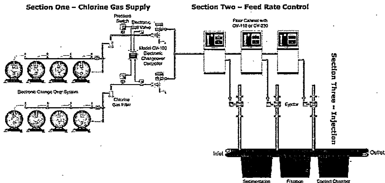
Figure 1: Surface Water Treatment Plant (Example)
