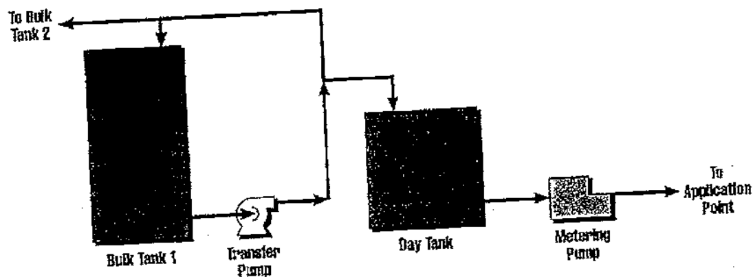
Figure ES-11 Liquid Chemical System Schematic
