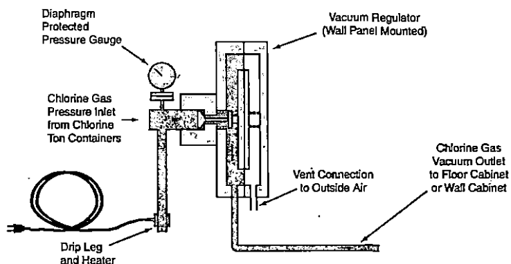
Figure 4: Vacuum Regulator
