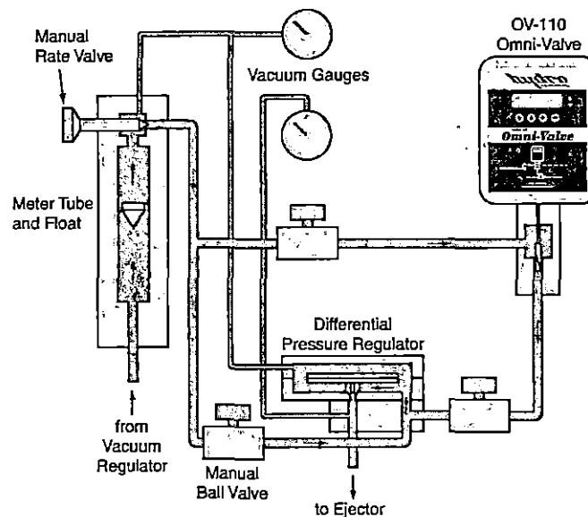
Figure 6: Feed Rate Control Equipment
