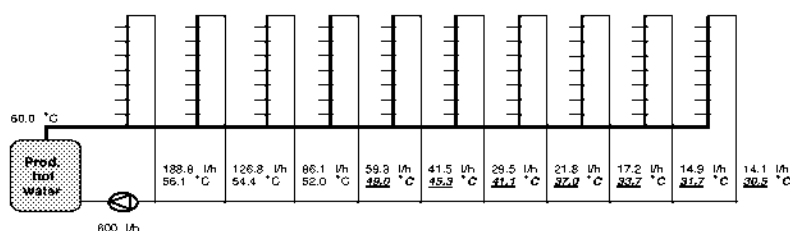
Example of unbalanced flow rates in a looped hot water system and its consequences on the temperature of circulated water
